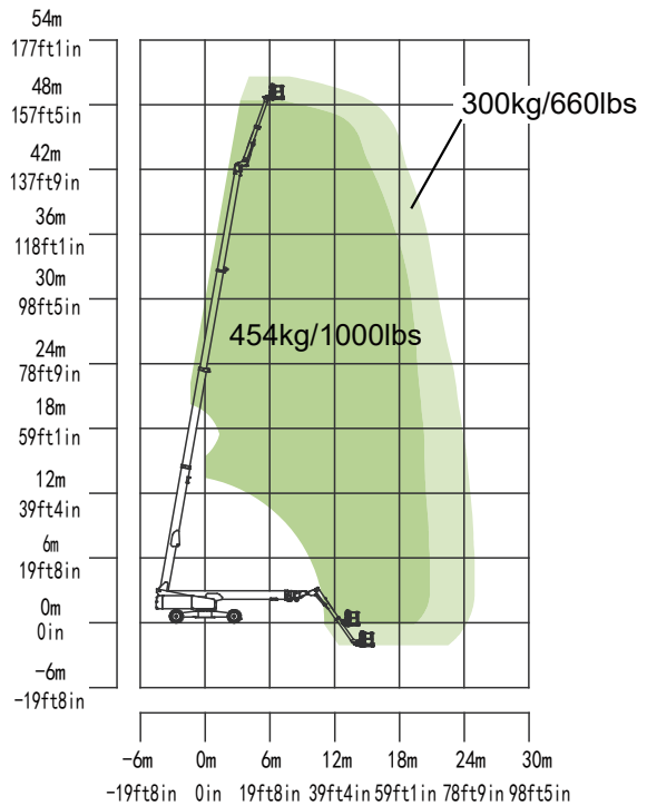
Range of Motion ZT51JEH-V
